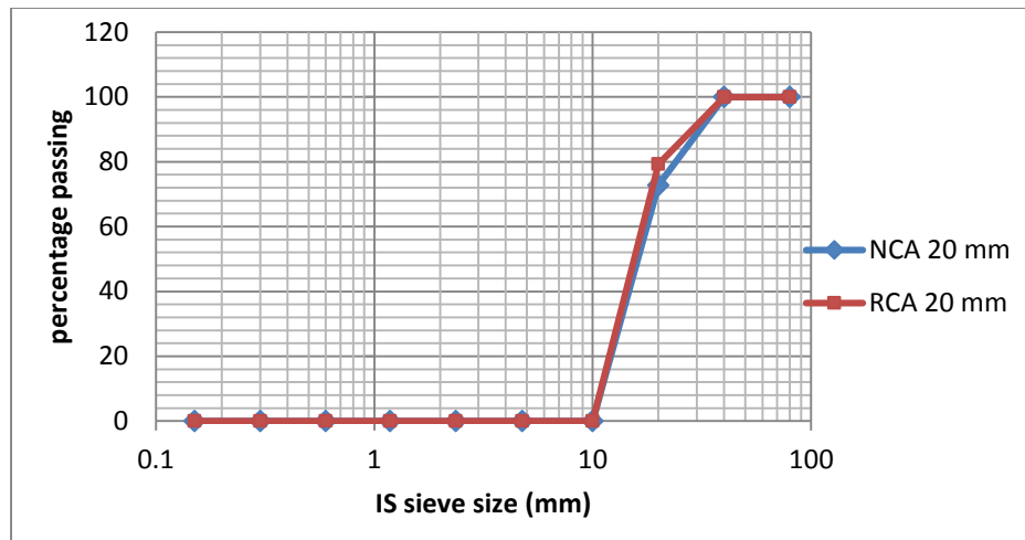
Figure 3: Grading Curves of Natural and Recycled Coarse Aggregate
