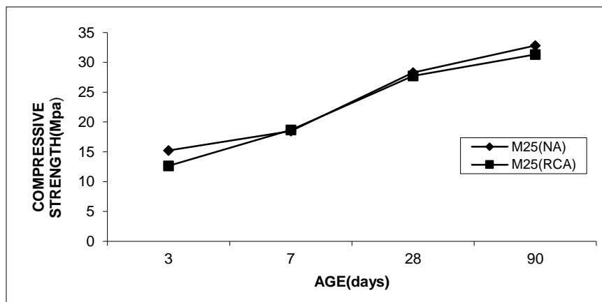
Figure 8: Variation of Compressive Strength of M 25 Grade Concrete with Curing Period
