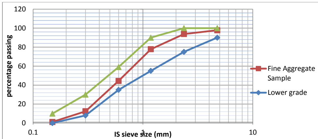
Figure 1: Grading Curve of Fine Aggregate
